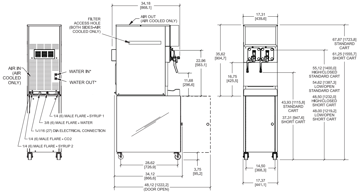
FIGURES IN BRACKETS INDICATE MILLIMETERS / DECIMAL AND FRACTIONAL DIMENSIONS EQUAL TO ( PLUS OR MINUS 1/16 INCH [1.5mm] / *WATER COOLED ONLY ).
