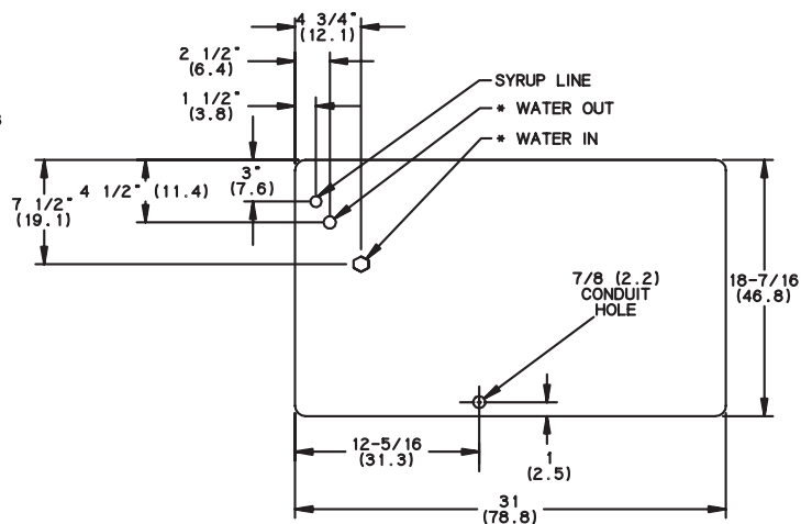
TOP VIEW BASE OPERATOR END
