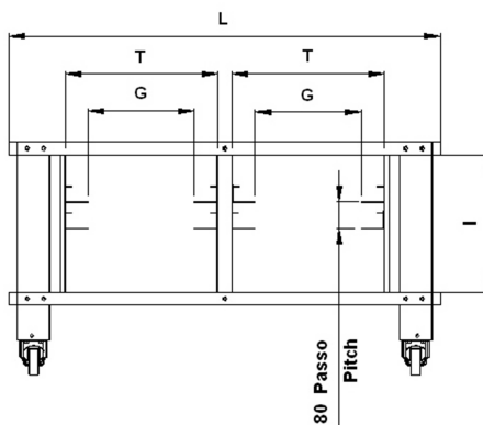
STAND REAR VIEW
