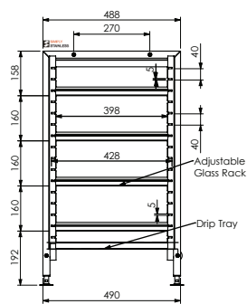
36-DGR SIDE ELEVATION
