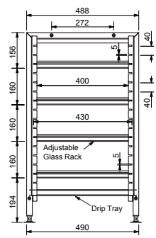
36-GR SIDE ELEVATION
