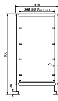
36-GR FRONT ELEVATION
