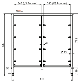
36-DGR FRONT ELEVATION
