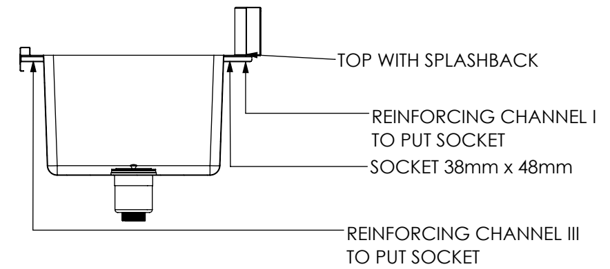
SECTION J-J
