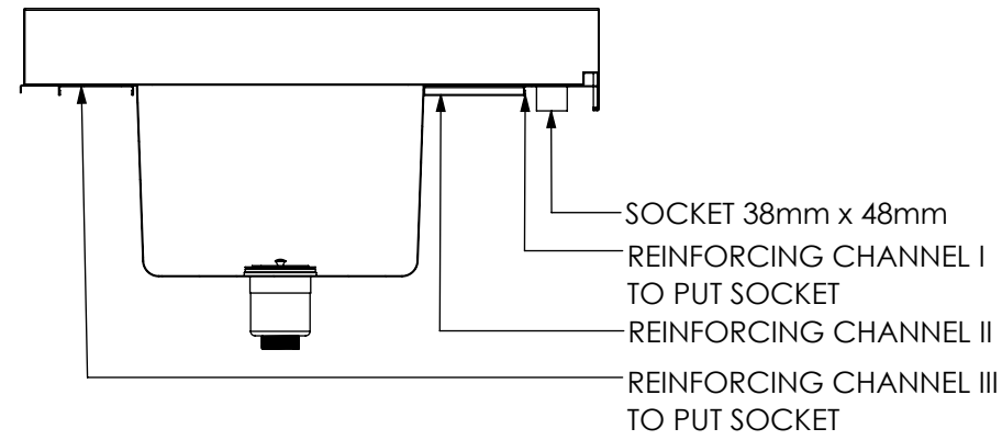
SECTION K-K
