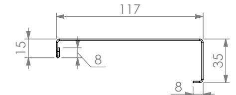
REINFORCING CHANNEL I DETAIL
