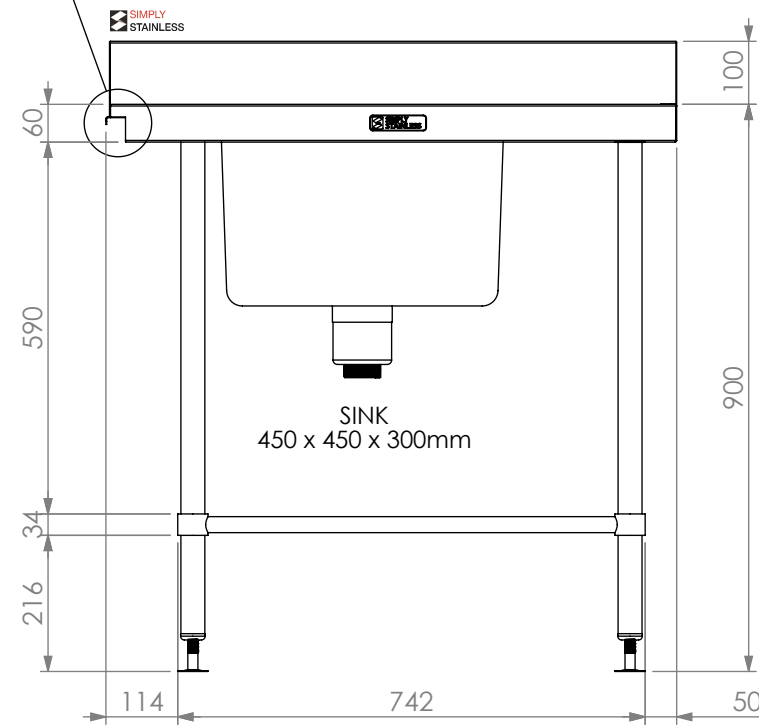
FRONT ELEVATION
