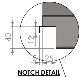
NOTCH DETAIL
