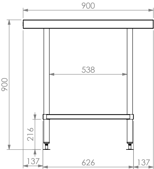
*900mm DEEP MODULE ELEVATION.
