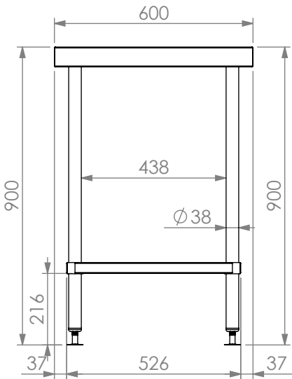
*600mm DEEP MODULE ELEVATION.
