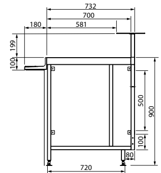
SIDE ELEVATION
