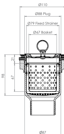
Cross Section
