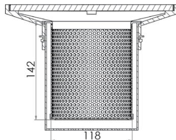
Cross Section
