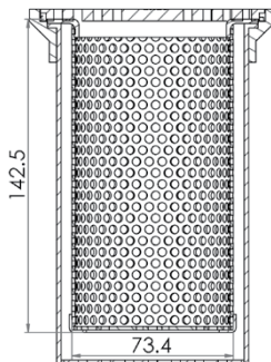
Cross Section
