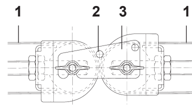
Transfer-table
