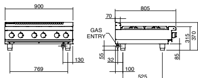
RNLB8600G-B
