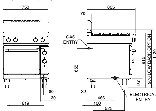
RN8510GEC, RN8513GEC
