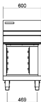
B60-CB Cabinet Base
