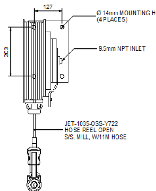
FRONT VIEW NPS
