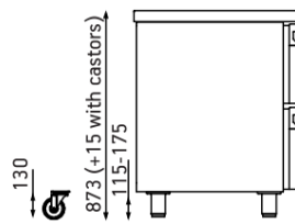
Castors will add 17mm to the height
