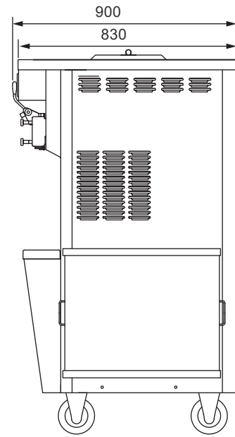
RIGHT SIDE
