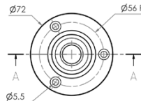
Mounting Body
