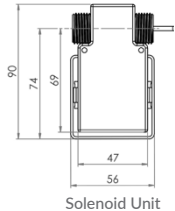
Solenoid Unit
