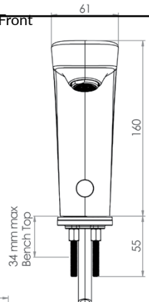
Solenoid Unit
