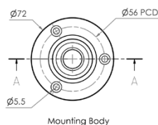
Mounting Body
