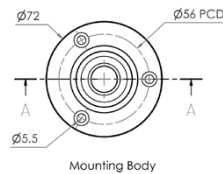
Mounting Body
