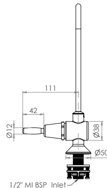
Front
