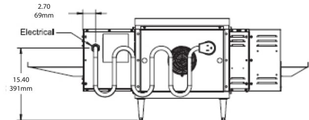
PS520 Back View – Electric, Single Unit
