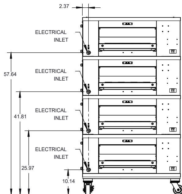
Side View – Quad Stacked with Casters
