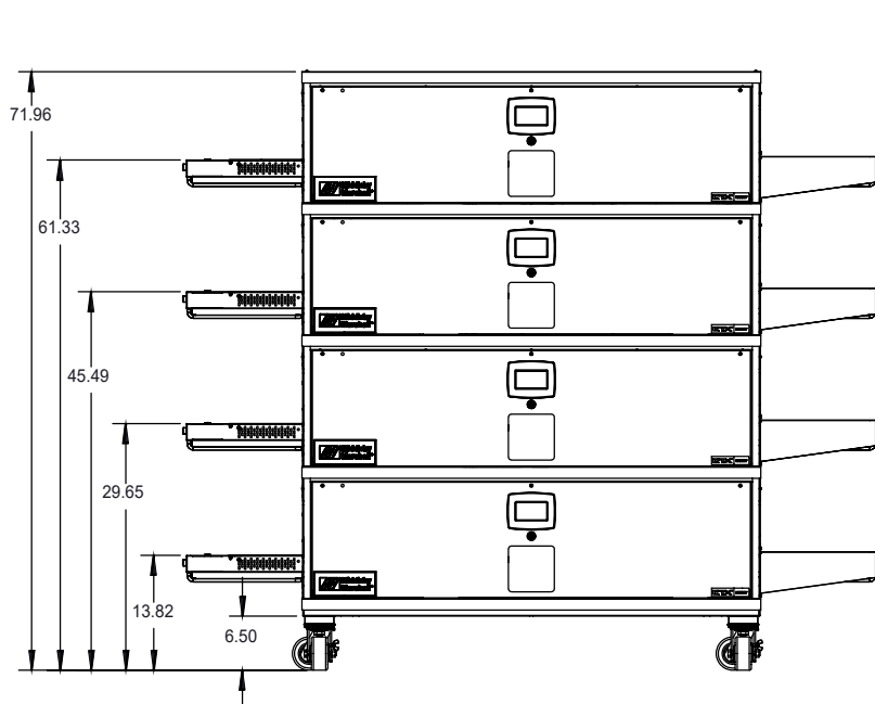
Front View – Quad Stacked with Casters
