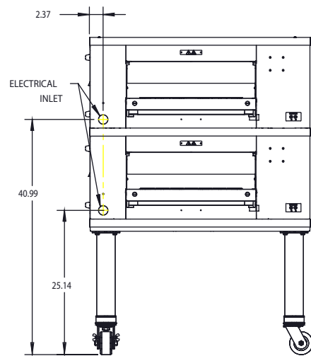
Side View – Double Stacked with 15" Legs
