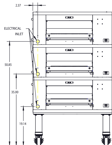
Side View – Triple Stacked with Casters
