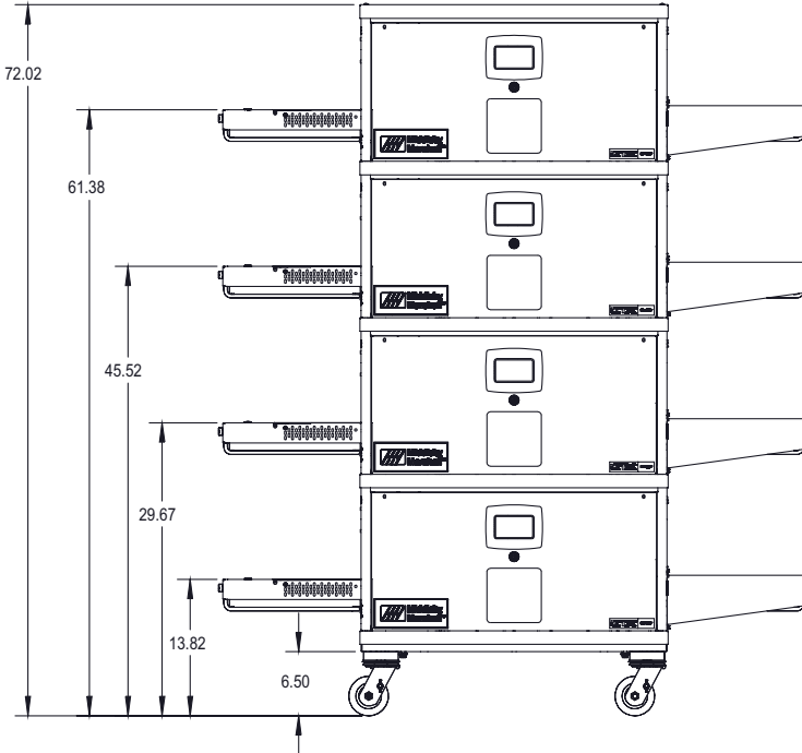
Front View – Quad Stacked with Casters
