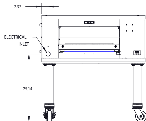
Side View with 15" Legs
