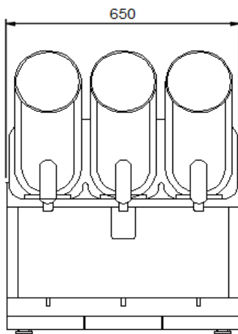
FRONT VIEW NTS
