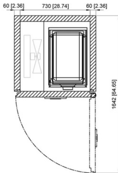
DIMENSIONS mm DIMENSIONS [in]
