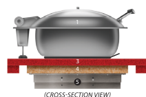
(CROSS-SECTION VIEW) 1. Chafing Dish 2. Magneeto™ 2 Trivet 3. Stone Countertop 4. Plywood Substrate 5. Incogneeto™ Unit
