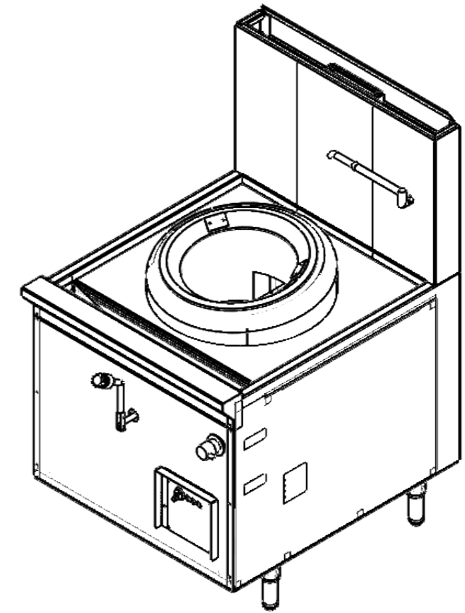
ISOMETRIC VIEW SCALE 1:15
