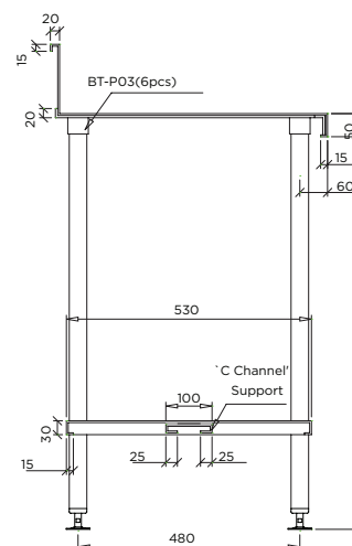
MODEL BT-WB-618 Section
