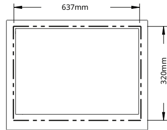
CUT-OUT DIMENSIONS
