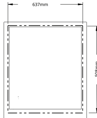
CUT-OUT DIMENSIONS
