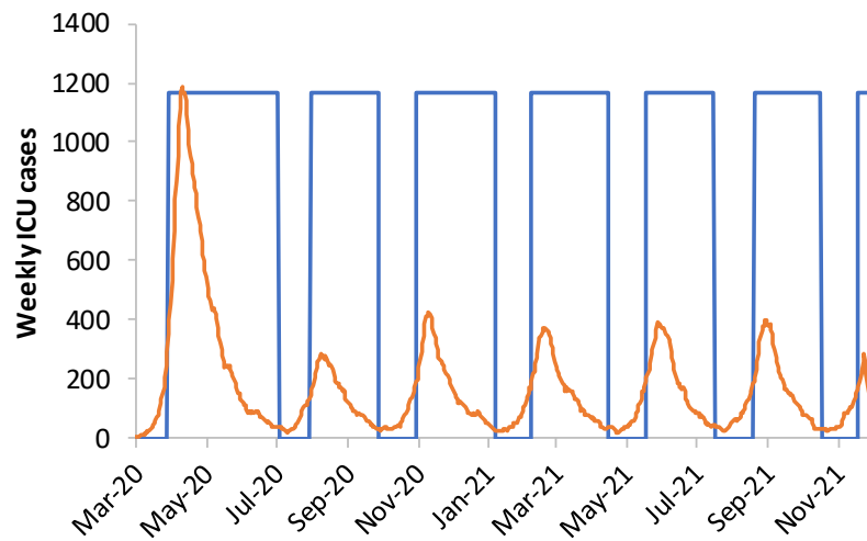
Figure 4: Illustration of adaptive triggering of suppression strategies in GB , for R_0=2.2 , a policy of all four interventions considered, an “on” trigger of 100 ICU cases in a week and an “off” trigger of 50 ICU cases. The policy is in force approximate 2/3 of the time. Only social distancing and school/university closure are triggered; other policies remain in force throughout. Weekly ICU incidence is shown in orange, policy triggering in blue.
