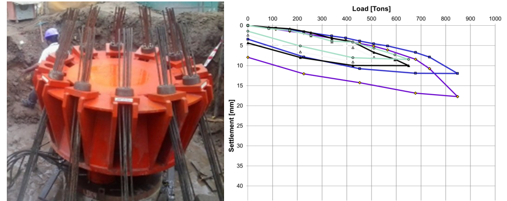
Figure 3: Crown system setup of rock anchors (left) Typical load v/s displacement curve for top-down testing of pile (right)
