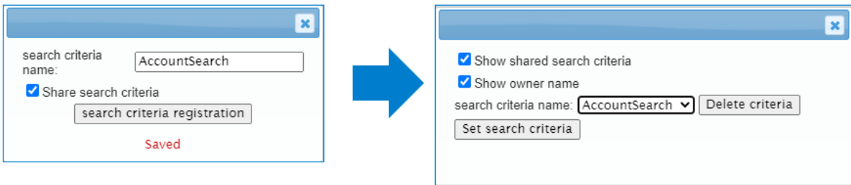
Figure 2-1 Save shared search criteria (left) and Load shared search criteria (right).
