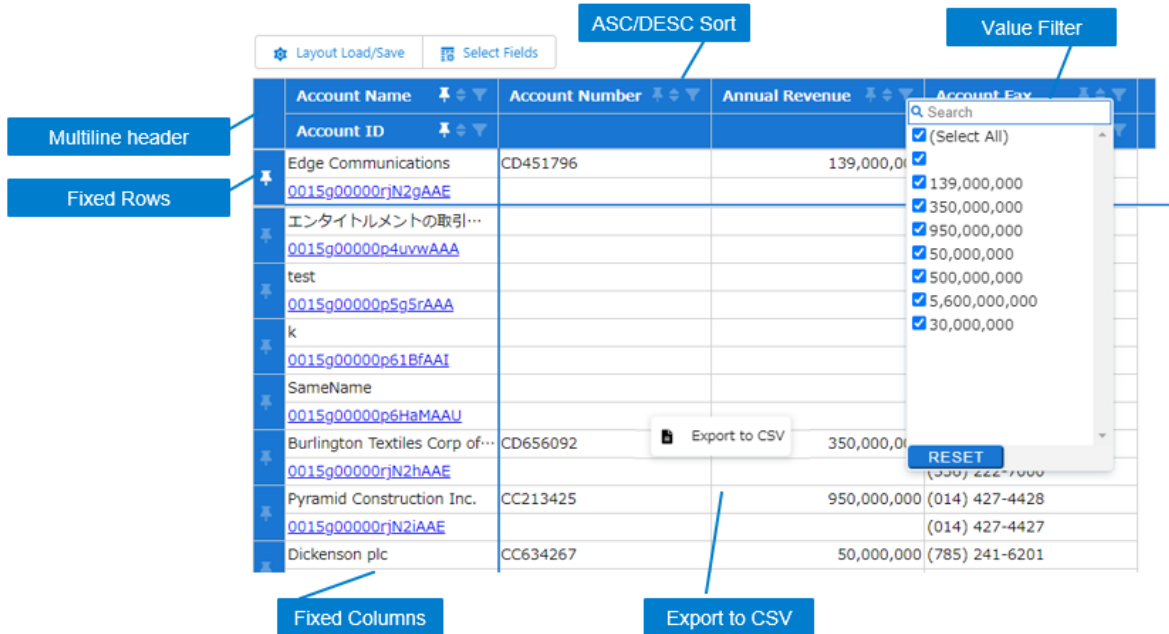
Figure 1-1 Examples of the various functions of Flexible Data Tables
