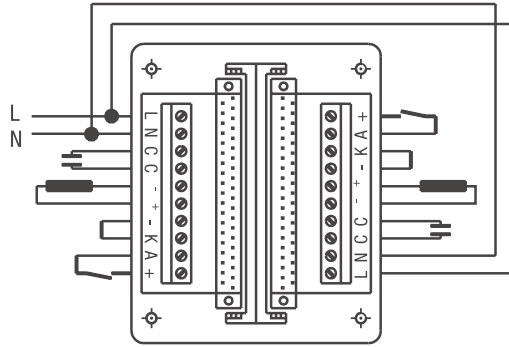
Control with two contacts
