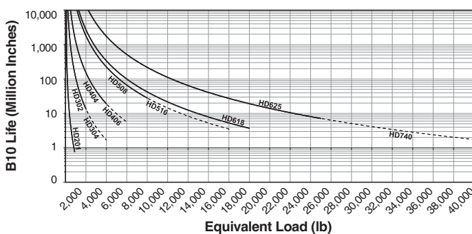
Dynamic Capacity: Life Vs. Load
