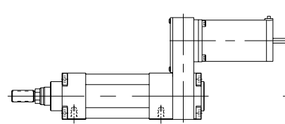
Reverse Parallel Mounting Positions (as viewed from the shaft end)
