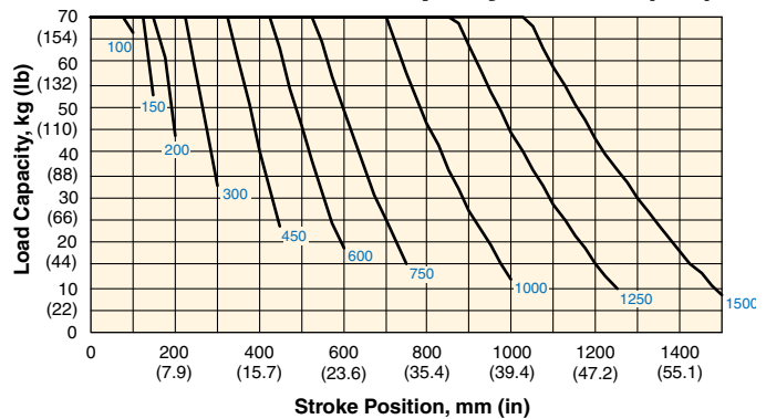
ET100 Rod End Load Capacity vs. Stroke (mm)
