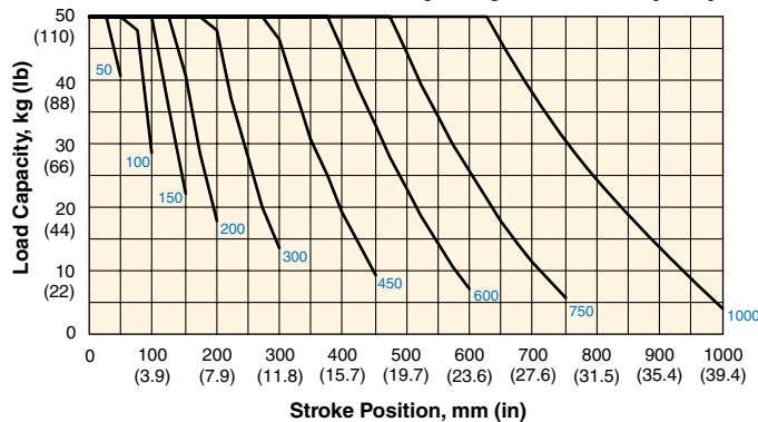
ET080 Rod End Load Capacity vs. Stroke (mm)
