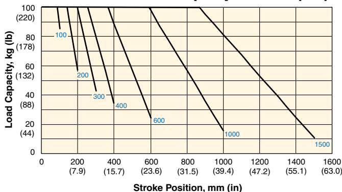
ET125 Rod End Load Capacity vs. Stroke (mm)
