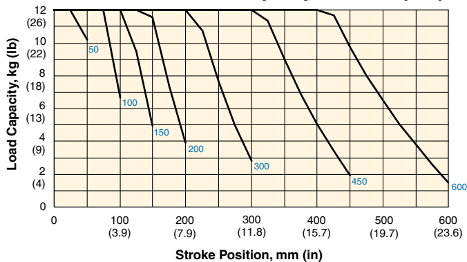
ET032 Rod End Load Capacity vs. Stroke (mm)
