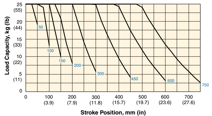
ET050 Rod End Load Capacity vs. Stroke (mm)
