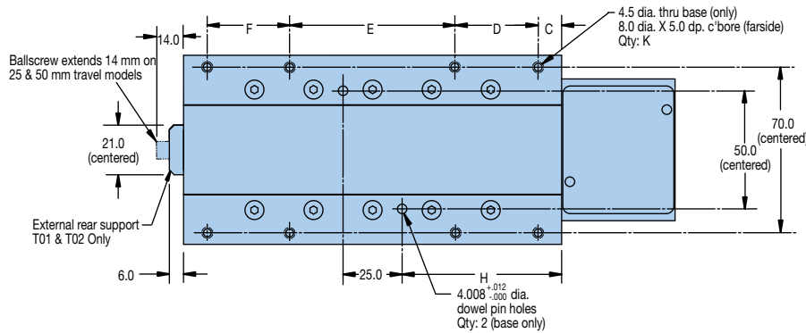
Dimensions (mm)
