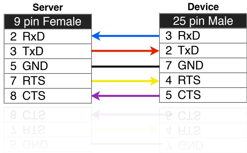
FIGURE 2.37: RS-232 9 to 25 pin straight through cable
