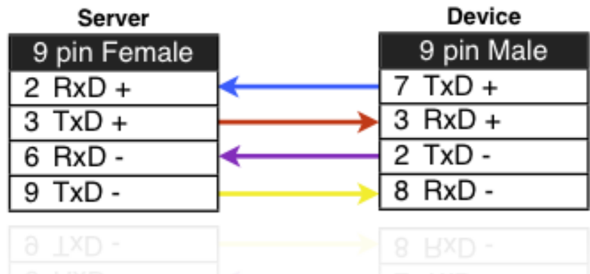
FIGURE 2.12: Qatech RS-422 cable
