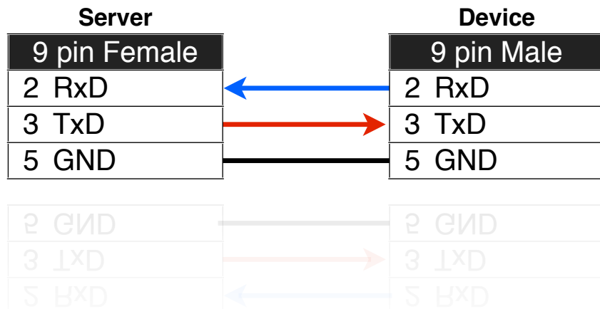
FIGURE 2.11: RS-232 straight through cable
