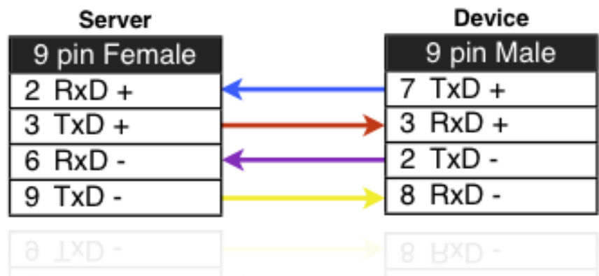
FIGURE 2.33: Qatech RS-422 cable
