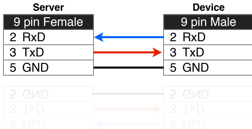
FIGURE 2.10: RS-232 straight through cable
