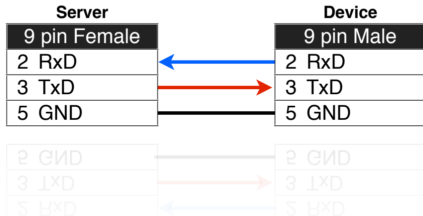
FIGURE 2.32: RS-232 straight through cable
