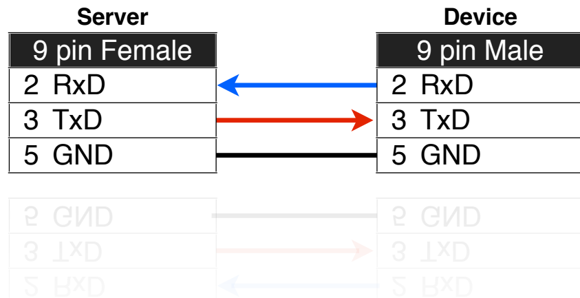
FIGURE 2.6: RS-232 straight through cable
