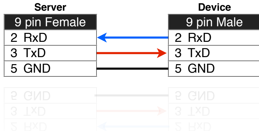
FIGURE 2.4: RS-232 straight through cable
