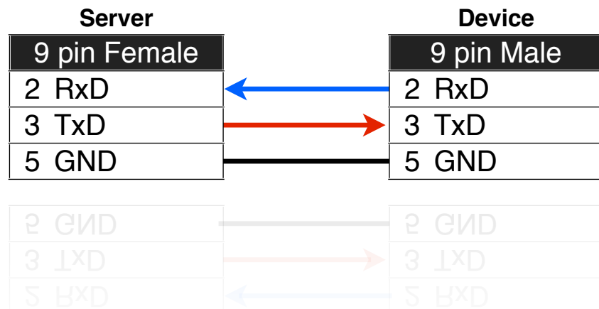
FIGURE 2.52: RS-232 straight through cable
