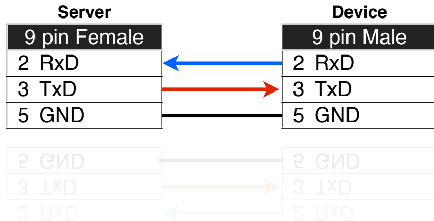
FIGURE 2.48: RS-232 straight through cable
