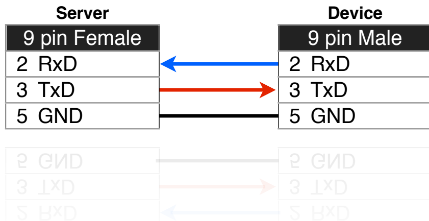
FIGURE 2.8: RS-232 straight through cable
