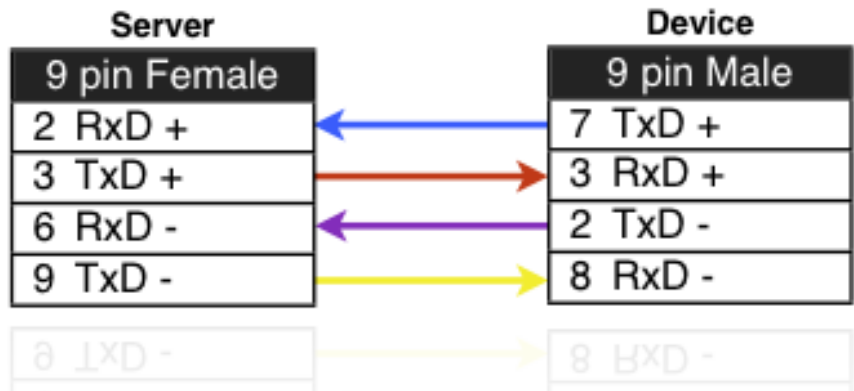
FIGURE 2.41: Quatech RS-422 cable
