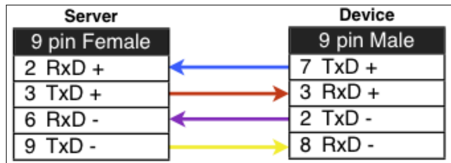
FIGURE 2.33: Quatech RS-422 cable
