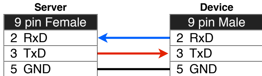
FIGURE 2.5: RS-232 straight through cable
