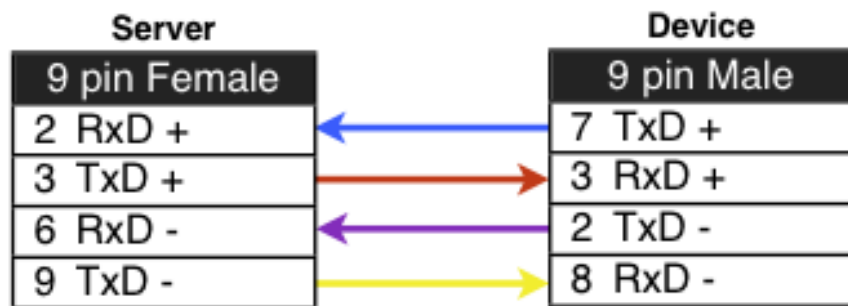
FIGURE 2.33: Qatech RS-422 cable
