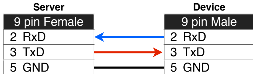
FIGURE 2.46: RS-232 straight through cable
