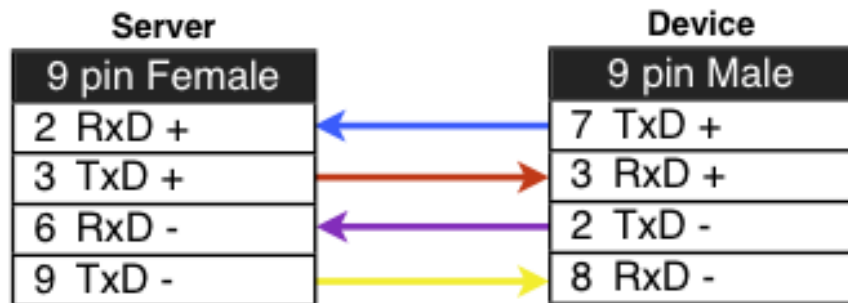
FIGURE 2.47: Quatech RS-422 cable
