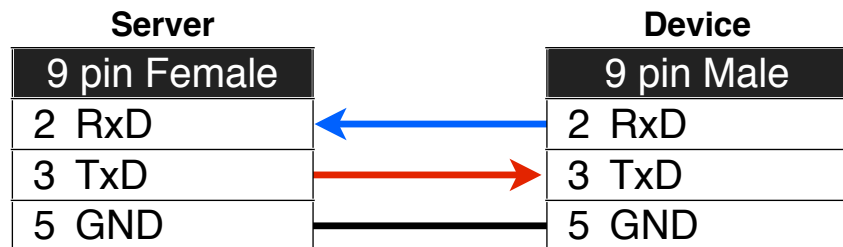
FIGURE 2.49: RS-232 straight through cable
