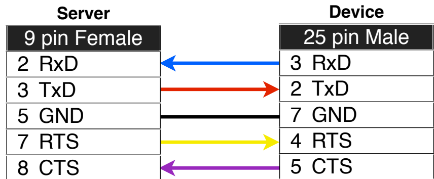
FIGURE 2.29: RS-232 9 to 25 pin straight through cable
