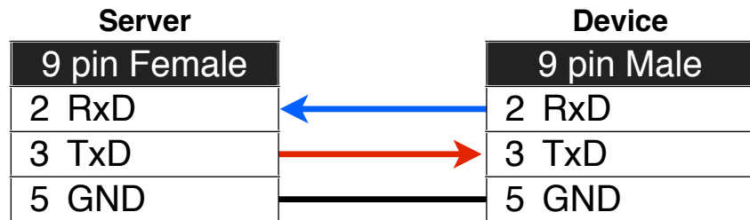
FIGURE 2.43: RS-232 straight through cable
