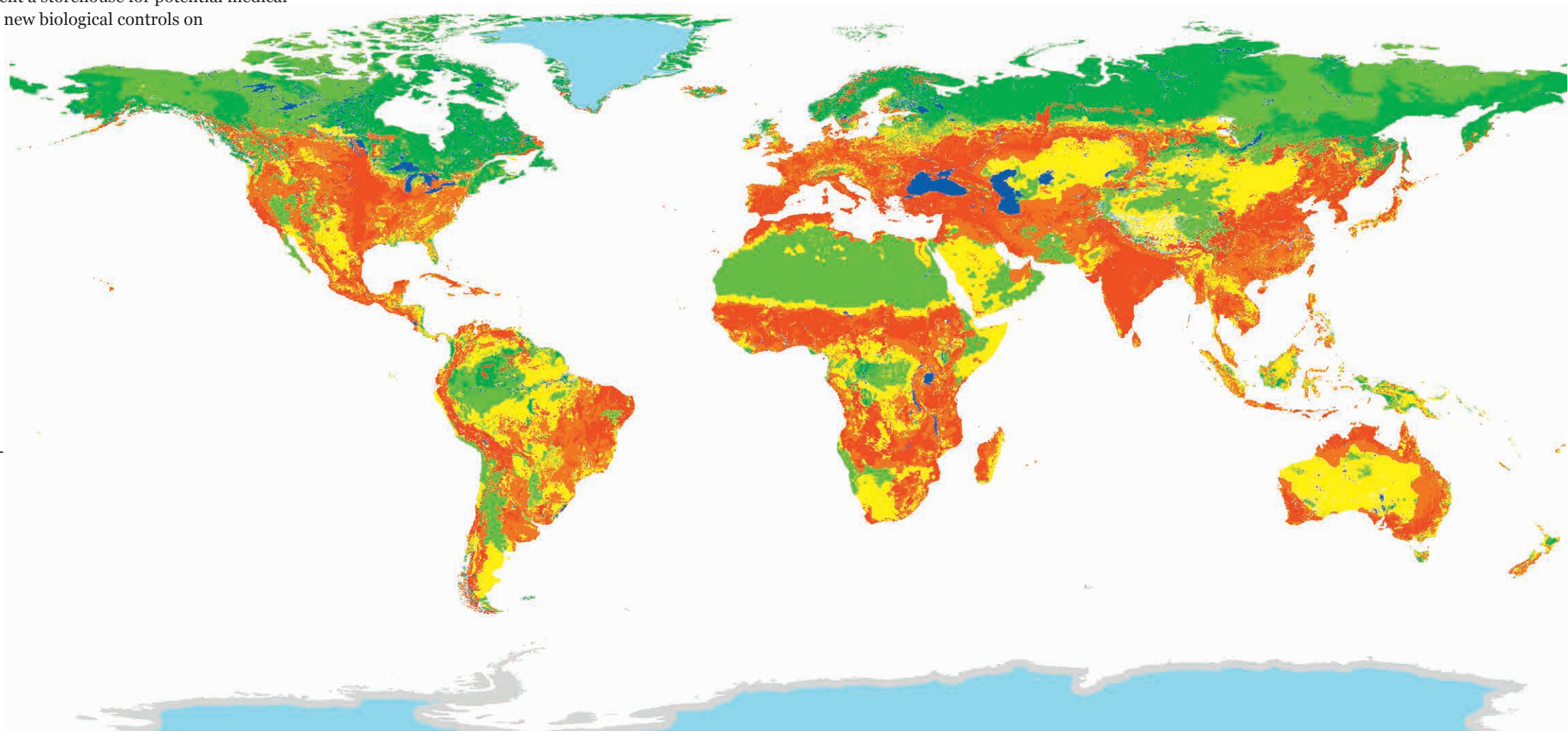
Figure 6: Global map showing the distribution of potential threats to soil biodiversity
