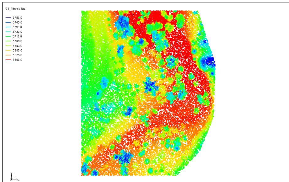
Figure 9 Filtered lidar
