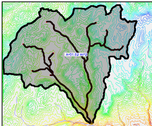
Figure 9 Delineated watershed basin showing streams
