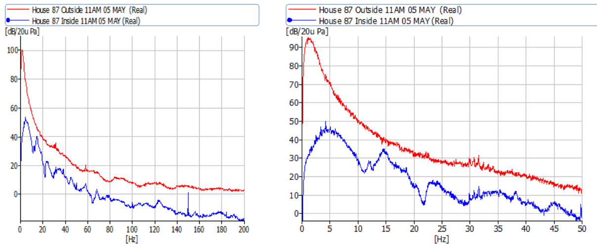
Figure 6: FFT
