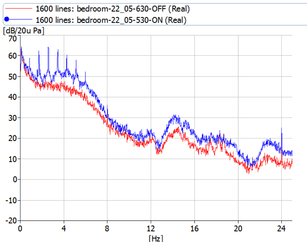
Figure 2 – Inside Bedroom
