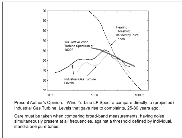
Figure 2. An example of low-frequency wind turbine spectrum Note. Reproduced with kind permission from Swinbanks (2010).
