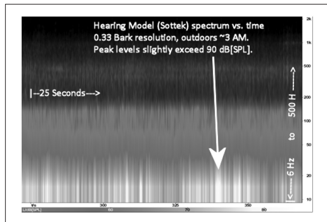
Figure 9. A spectrogram of infrasonic emissions Note. Reproduced with kind permission from Wade Bray, Head Acoustics.
